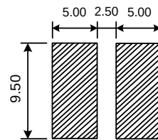
Recommended Land Pattern (mm)
